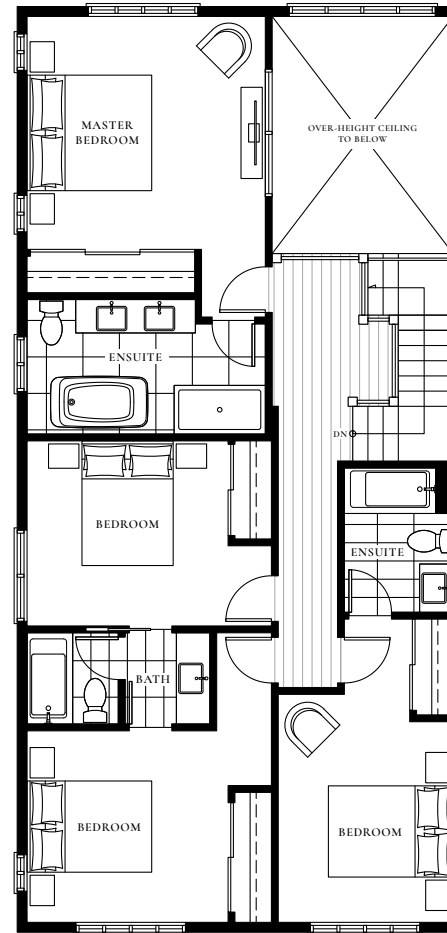
2 ND FLOOR
